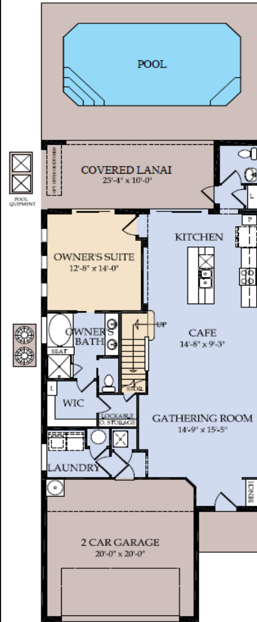
FIRST FLOOR
